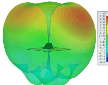
Typical 3D Pattern - 900MHz
