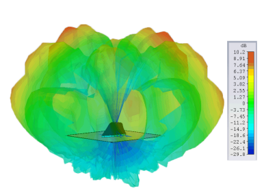
Typical 3D Pattern 5500MHz
