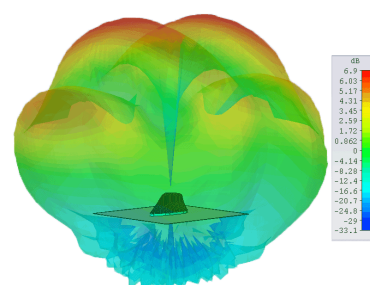
Typical 3D Pattern 2500MHz
