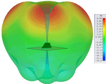
Typical 3D Pattern - 700MHz
