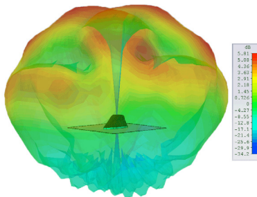
Typical 3D Pattern 2100MHz
