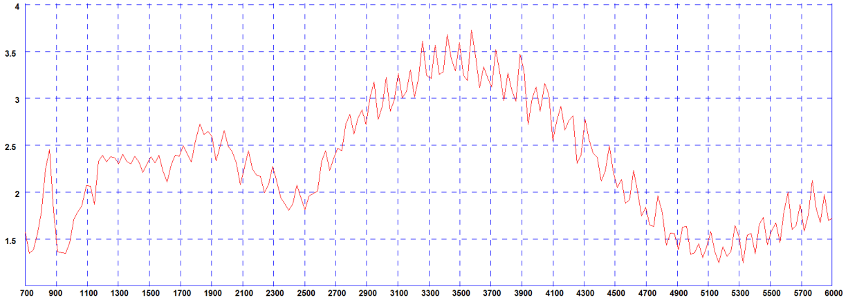
Typical VSWR*
