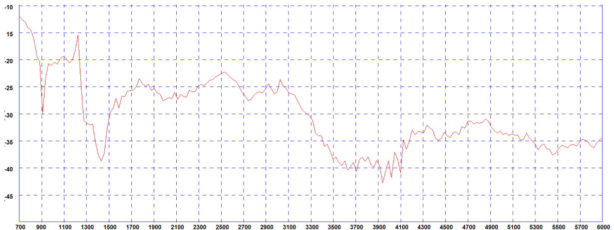
Typical Isolation *
