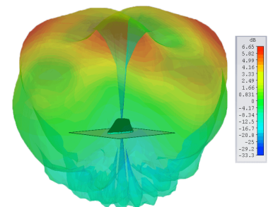
Typical 3D Pattern - 1800MHz
